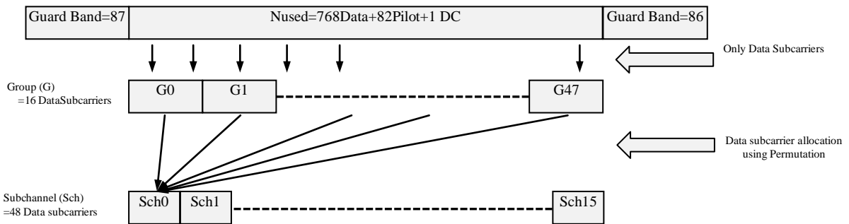
Figure (3): Distributed permutation process of DL FUSC (1024-FFT)
