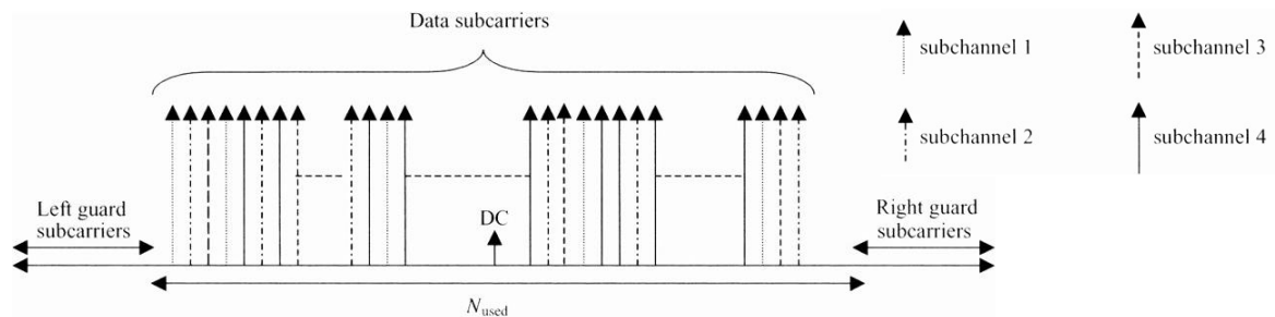
Figure (1): OFDMA frequency description (4 sub channel schematic example)
