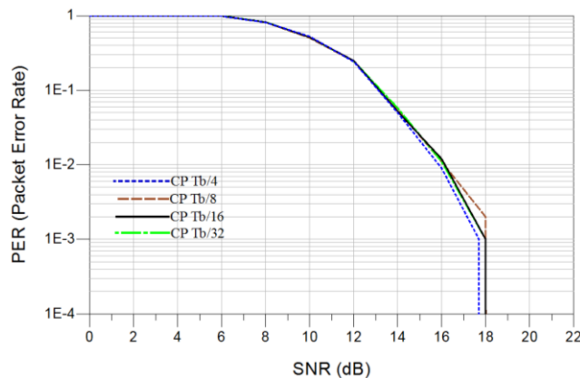
Figure (9): PER vs. SNR for FUSC mode - different CP values
